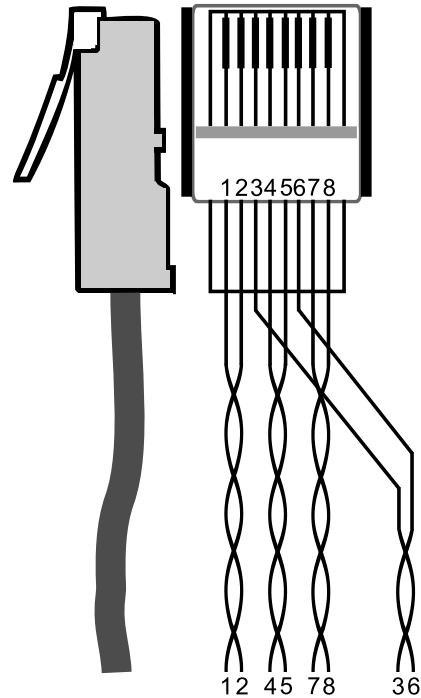
Figure 4: CAT5 PINOUT
