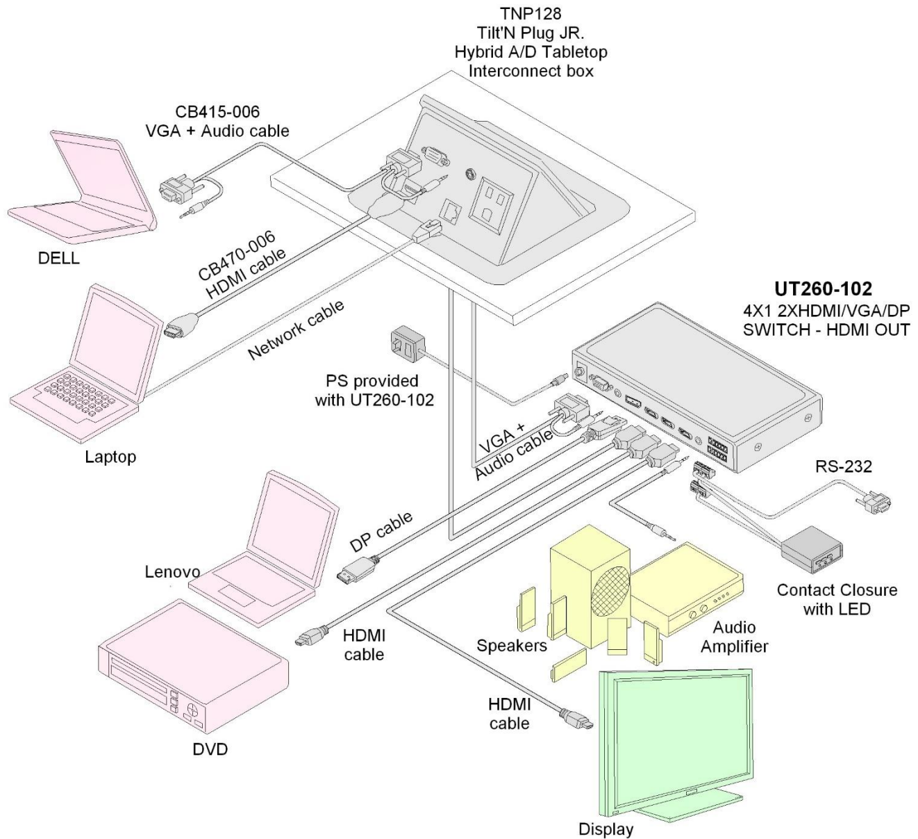
Diagram 1: Typical Setup
