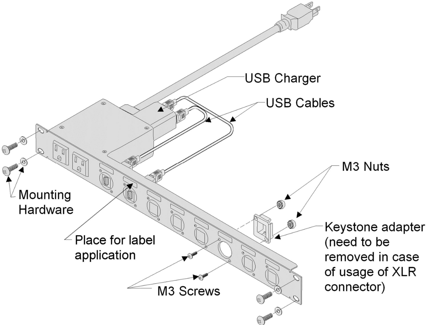
Diagram 3: Installation Diagram
