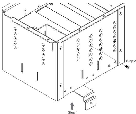
Figure 6: Installing the T-TBLANK TOOL Blank
