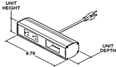
2 RECEPTACLES 1 TELECOM PLATE KNOCKOUT
