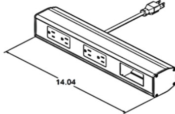
4 RECEPTACLES 1 TELECOM PLATE KNOCKOUT
