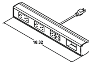
6 RECEPTACLES DUAL USB-C® PORTS 1 TELECOM PLATE KNOCKOUT
