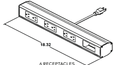
6 RECEPTACLES 1 TELECOM PLATE KNOCKOUT
