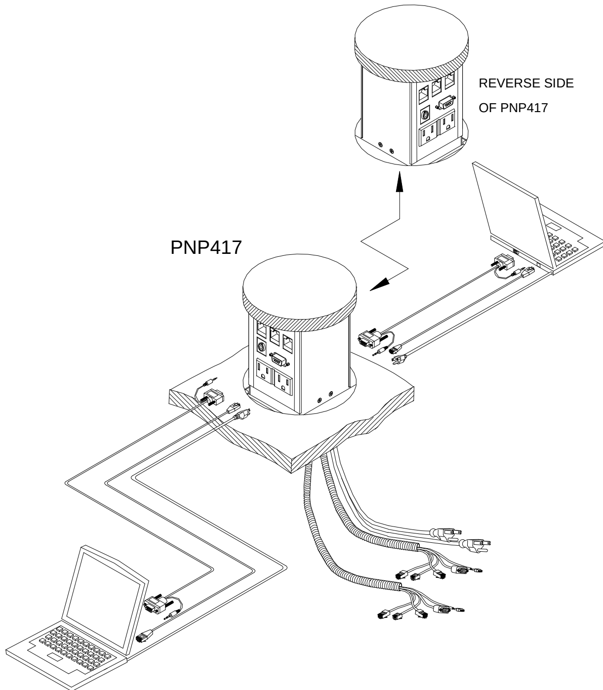
Diagram 1: Typical Setup
