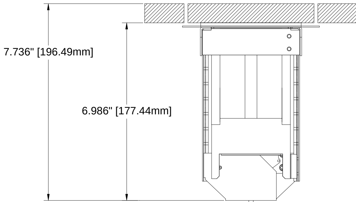
Diagram 3: Closed Dimensions
