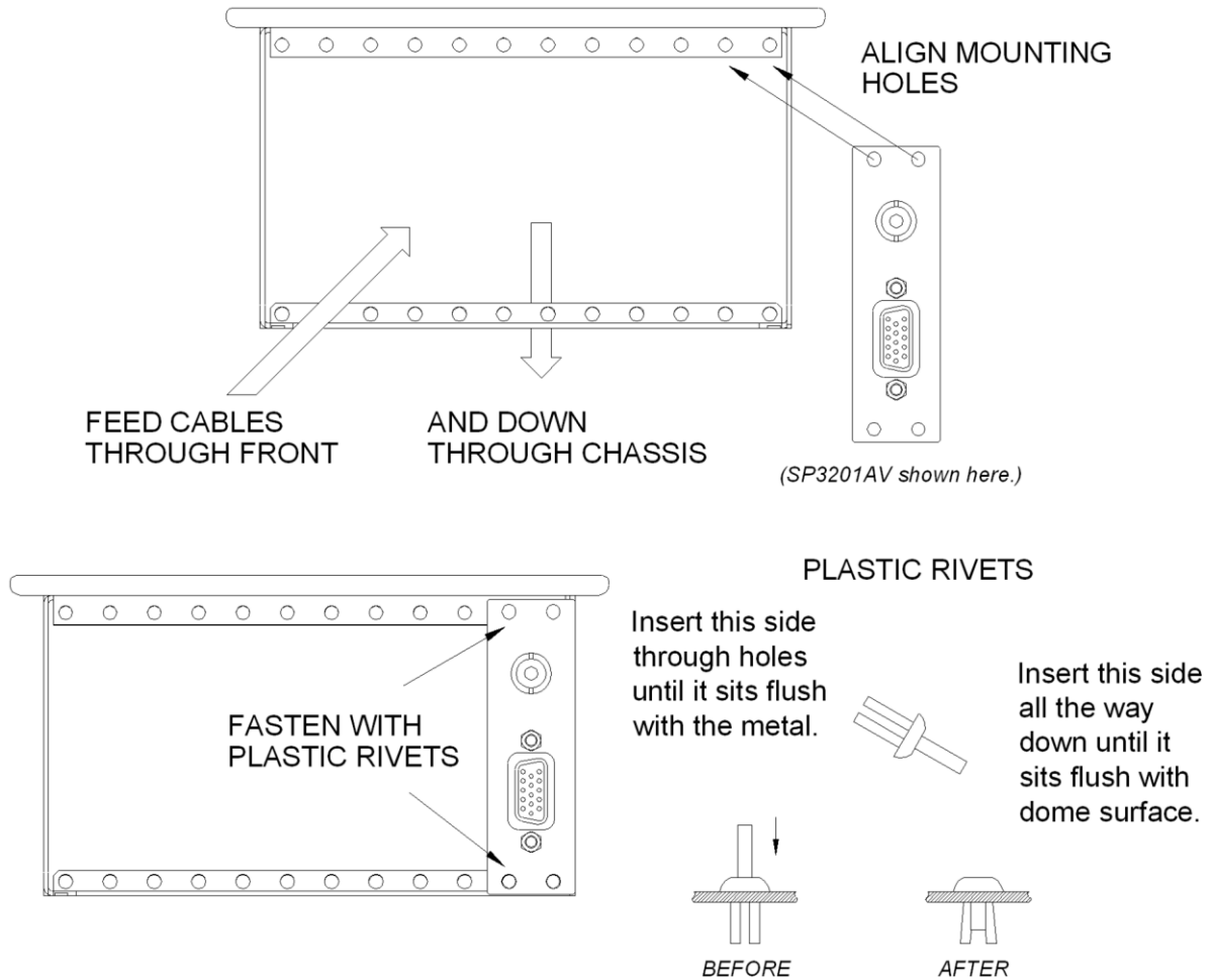
Diagram 7: Accessory Installation
