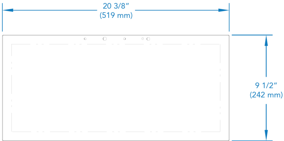
MXD-2001-PAN (Front View)
