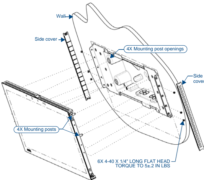
FIG. 5 MXD-2001-PAN installation (Landscape)
