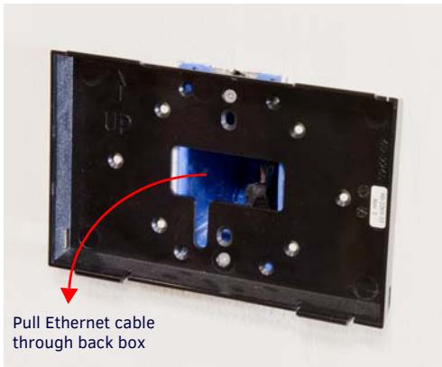
FIG. 6 ACCESSING THE ETHERNET CABLE THROUGH THE BACK BOX.
