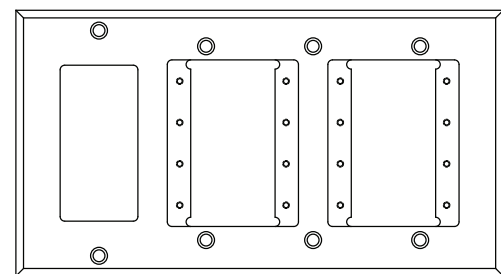
IPS-WP3Q 2 IPS & 1 Decora Opening
