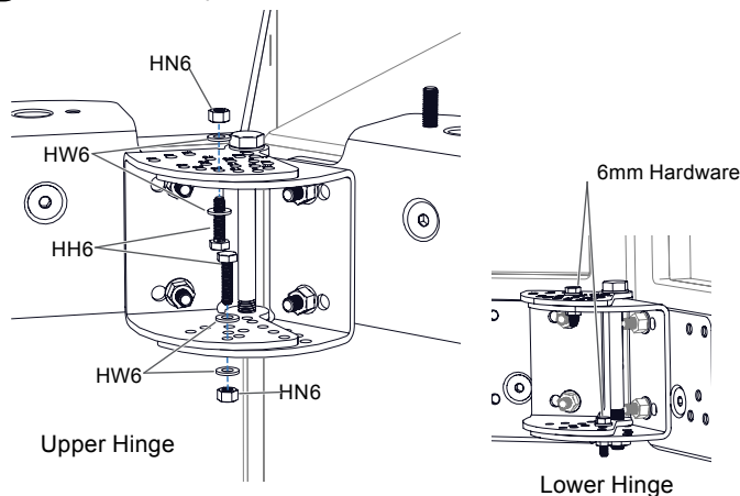
Figure 24-6H. Secure angle on hinges by reinserting the 6mm hardware removed earlier Snug tighten the 6mm connections until desired angle is confirmed, then fully tighten
