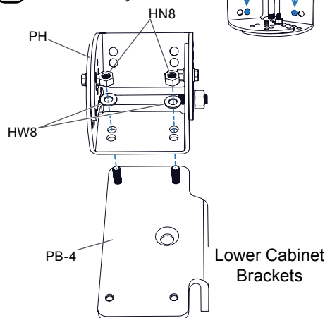
Figure 24-4V (Vertical Array). Remove the 6mm hardware from the hinges and attaching the lower cabinet brackets to the hinge assemblies, and then to the cabinet brackets on the suspended cabinet (build from the top > down)
