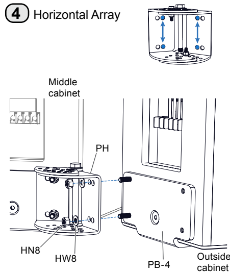
Figure 24-4H (Horizontal Array). Remove the 6mm hardware and connect the hinge assemblies to the cabinet brackets (build from the inside-out)
