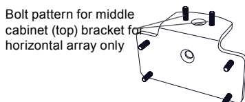
Figure 24-1. 8mm flat head bolt positions in cabinet brackets by kit application. (Lightly shaded outlined items are included in the HVS3 kit) Brackets are shown in their orientation on the full-range cabinets.
