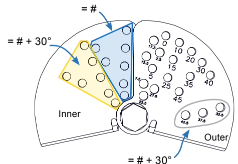
DFS kit shown with 2 IP6/IP8-1122s 30° splay shown which also equals the center-to-center measurement
