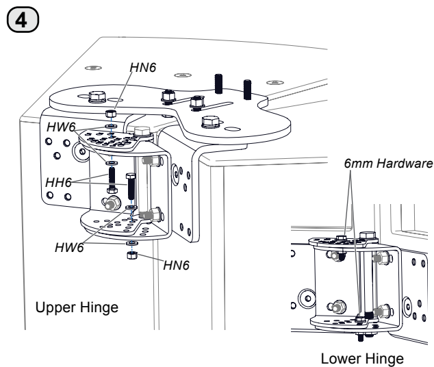
Figure 4. Secure angle on hinges by reinserting the 6mm hardware removed earlier - snug tighten
