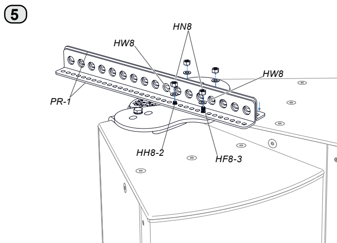
Figure 5. Remove the locknuts and flat washers from the hex head bolts in the adapter plate, move the bolts to the back of the slots , and attach the fly rails
