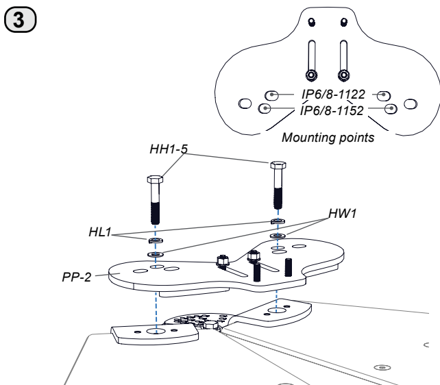
Figure 3. Attach splay plate - snug tighten bracket connections
