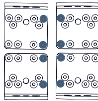
Figure 1a. After removing the applicable cabinet bolts, place cabinet brackets (with flat head bolts inserted) on the cabinets as shown
