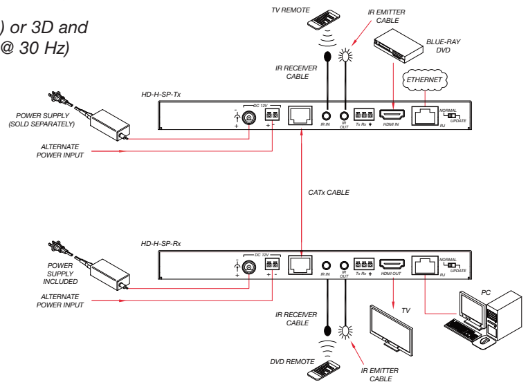
Application example using an HD-H-SP-Tx and HD-H-SP-Rx shown. Refer to specific model information for full features.
