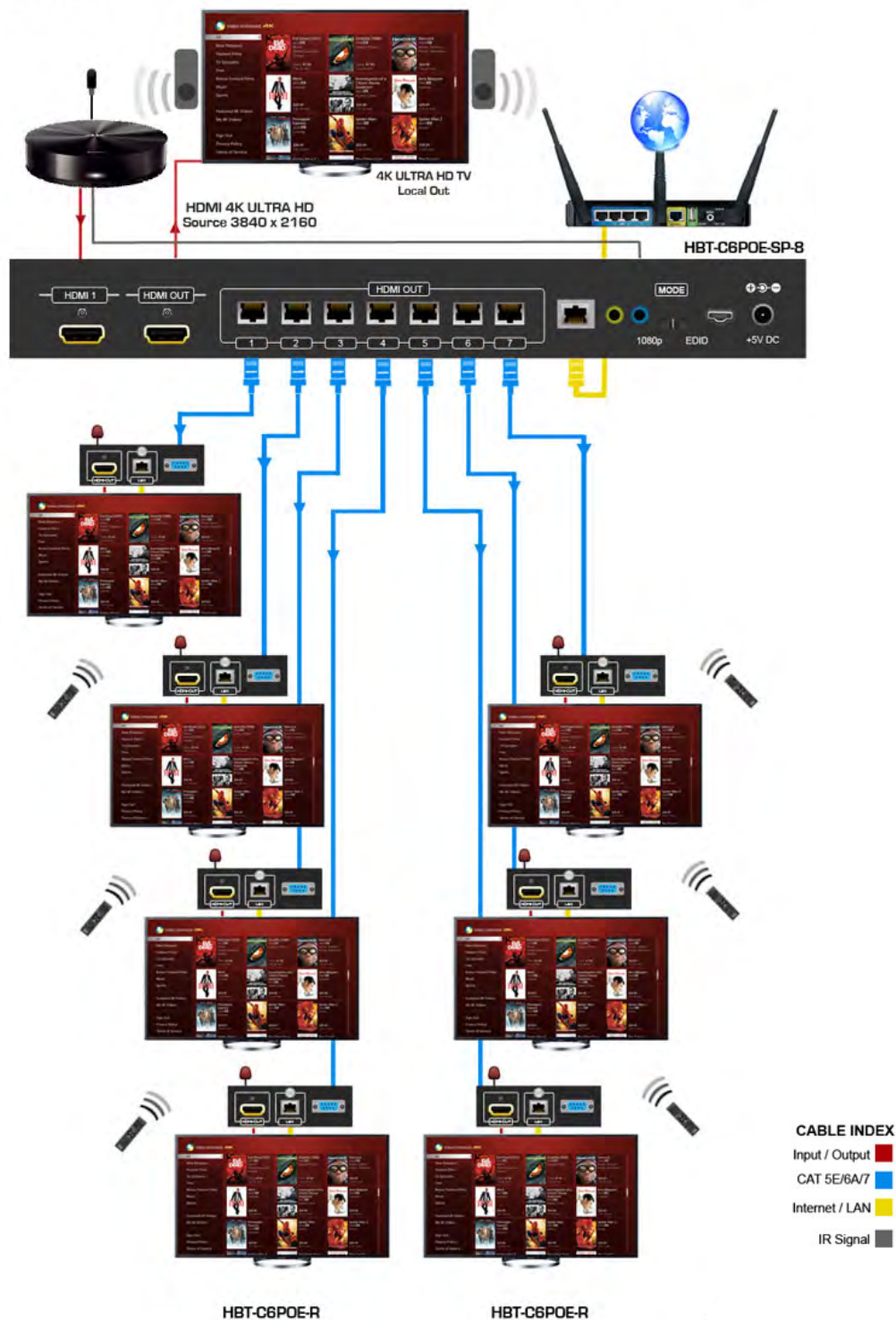
LAYOUT 1
