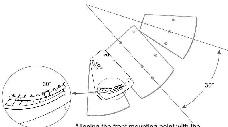
Figure 1. Attach universal mounting plates to subwoofer
