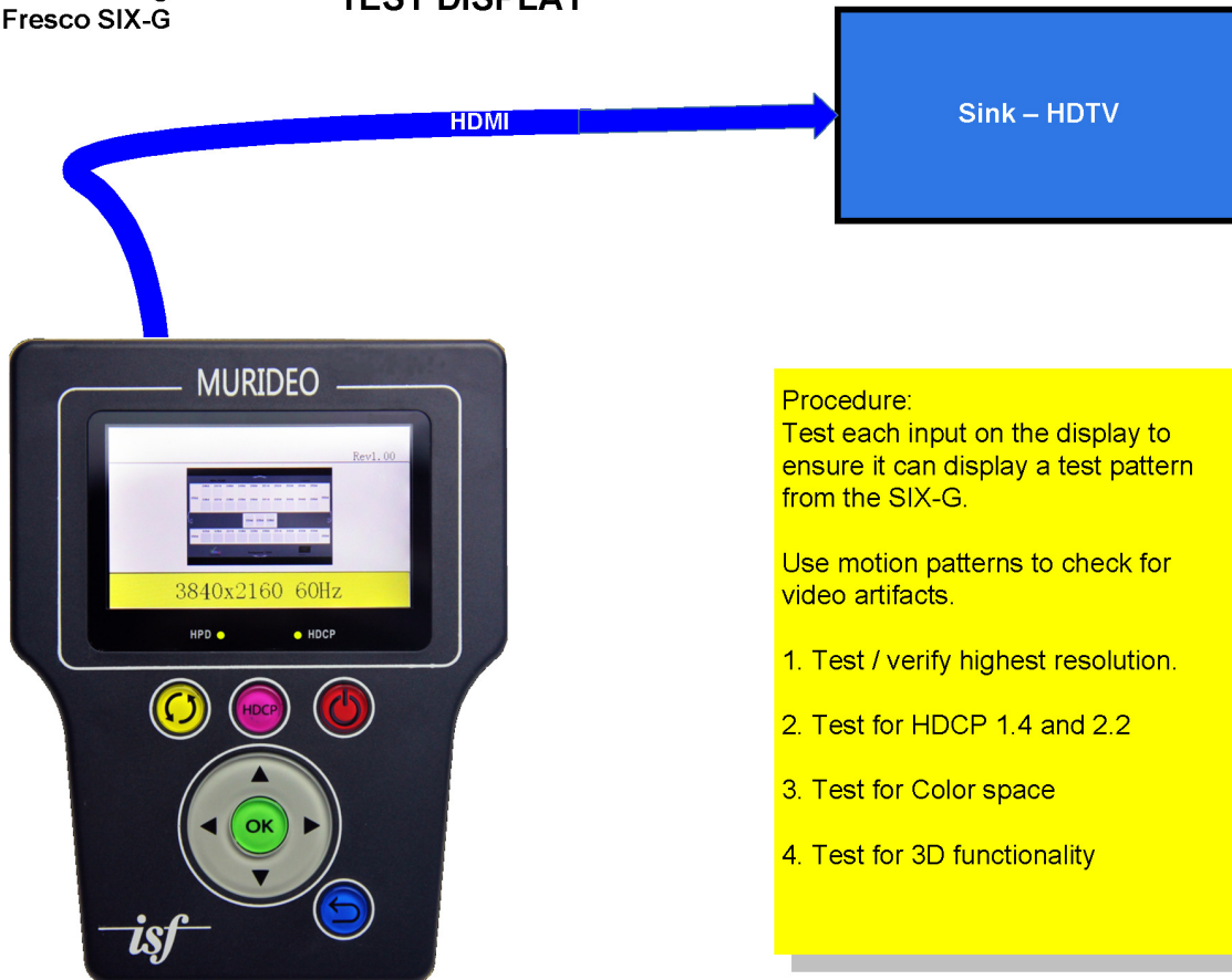
Connection Diagram Fresco SIX-G
