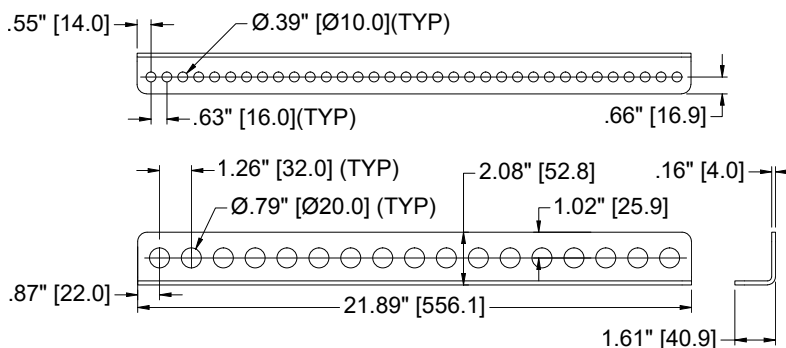
Cabinet Corner Bracket (2-WAY) [PB-3]
