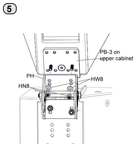
Figure B-5. Remove 6mm hardware (securing the angle) and attach hinge to the cabinet bracket on the upper cabinet
