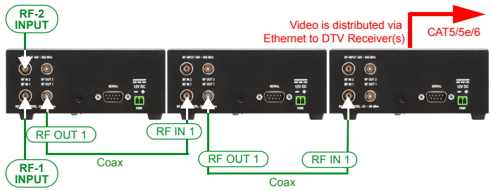
FIG. 4 RF OUT 1/2
