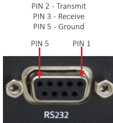
DL-HD24A-H2 DB9 FEMALE
