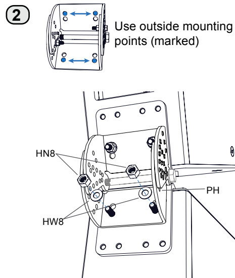
Figure 2. Remove 6mm hardware (securing the angle) and attach the hinge to the upper cabinet and then the lower one - leave connections loose until both cabinets have been connected
