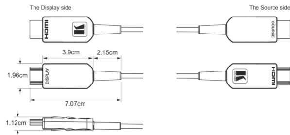
Figure 1: HDMI Connectors – SOURCE and DISPLAY (with Dimensions)
