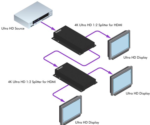
Figure 1.1 - Using two 1:2 Splitter units to distribute an Ultra HD source to three Ultra HD displays
