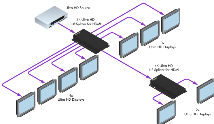
Figure 1.2 - Using a 1:8 Splitter and a 1:2 Splitter to distribute an Ultra HD source to nine Ultra HD displays
